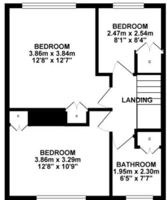
1ST FLOOR 41.44 sq. m. ( 446.00 sq. ft. )
